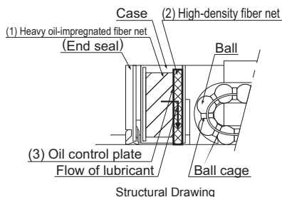
Structural Drawing
