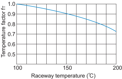
Fig.9 Temperature Factor (f T )
