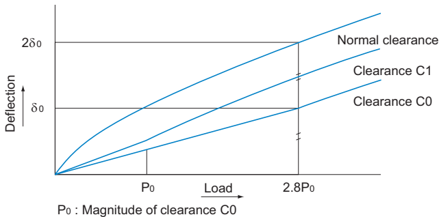
Fig.14 Rigidity Data
