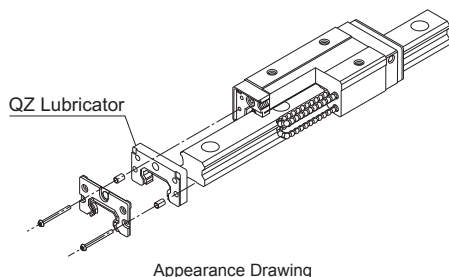
Appearance Drawing
